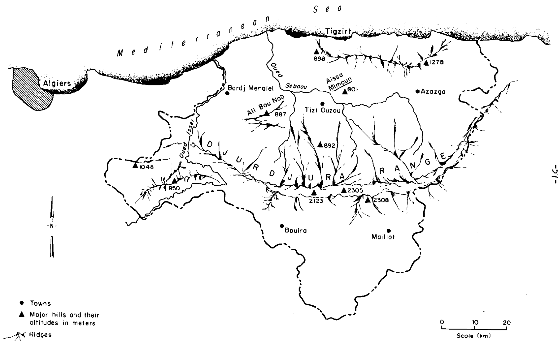
Fig. 2—Terrain features of Greater Kabylia
